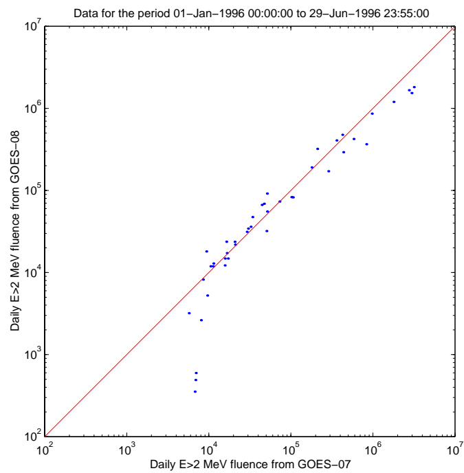
Figure 2.8: A correlation plot for the GOES-7 and GOES-8 > 2 MeV daily electron fluence for the first half year of 1996. The data are one day fluence values and the units are \text{cm}^{-2} \text{sr}^{-1} .
