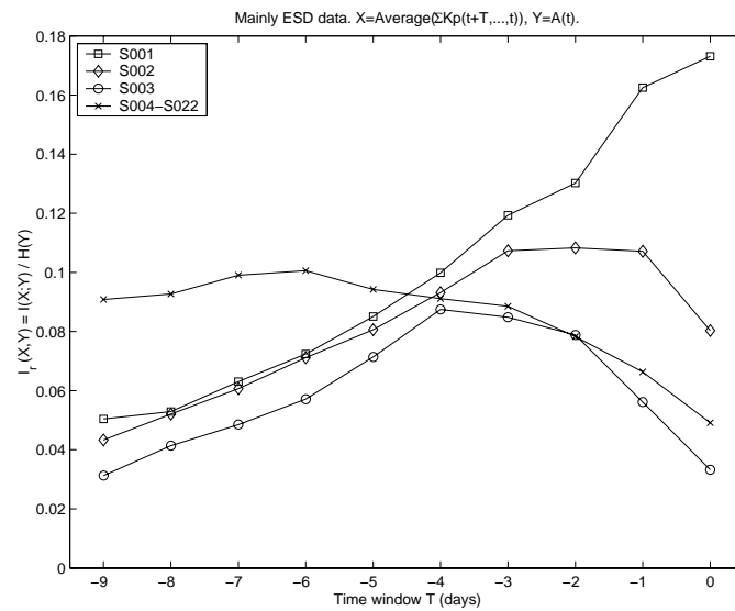
Figure 2.2: The relative mutual information I(X;Y)/H(Y) for the different anomaly sets as a function of the average \sum K_p , where the average goes from 1 to 10 days. A subset of the anomaly data is selected that mainly related to ESD as explained in the text.
