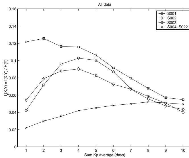
Figure 2.1: The relative mutual information I(X; Y)/H(Y) for the different anomaly sets as a function of the average \sum K_p , where the average goes from 1 to 10 days. The anomaly sets contain all the anomaly data.
