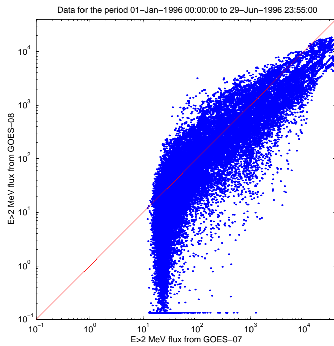
Figure 2.7: A correlation plot for the GOES-7 and GOES-8 > 2 MeV electron flux for the first half year of 1996. The data are 5 minute averages and the units are \text{cm}^{-2} \text{s}^{-1} \text{sr}^{-1} .
