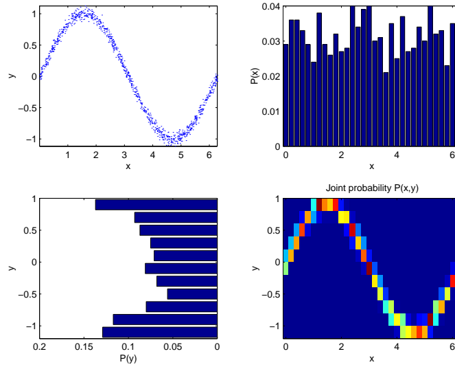
Figure 3.1: A sine curve y = \sin x (top left) and the probabilities p(x) (top right) and p(y) (bottom left) using a bin size of 0.1, and the joint probabilities p(x, y) (bottom right).
