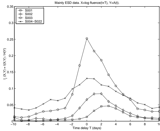
Figure 2.4: The relative mutual information I(X; Y)/H(Y) for the different anomaly sets as a function of log daily > 2 MeV electron fluence delayed -10 to 10 days. A subset of the anomaly data is selected that mainly related to ESD as explained in the text.
