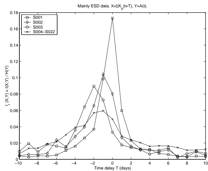
Figure 2.3: The relative mutual information I(X;Y)/H(Y) for the different anomaly sets as a function of \sum K_p delayed -10 to 10 days. A subset of the anomaly data is selected that mainly related to ESD as explained in the text.
