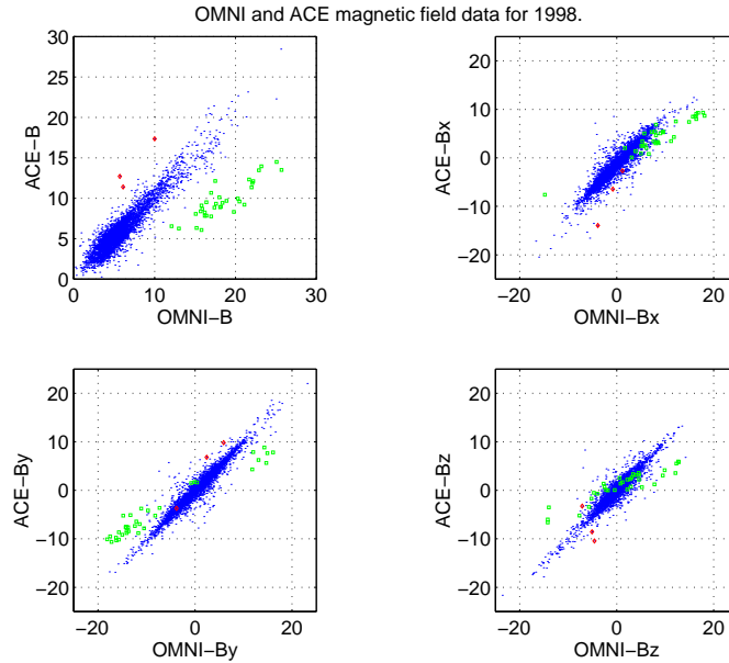
Figure 2.6: Correlation plots between the hourly OMNI magnetic field data and the ACE magnetic field data over the year 1998. The figures show the magnitude of the average magnetic field ( B ), and the magnetic field components ( B_x, B_y, B_z ).
