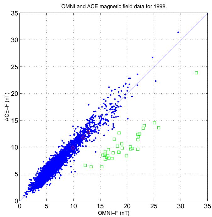
Figure 2.5: Correlation plots between the hourly OMNI magnetic field data and the ACE magnetic field data over the year 1998. The figure shows the average field magnitude ( F ).
