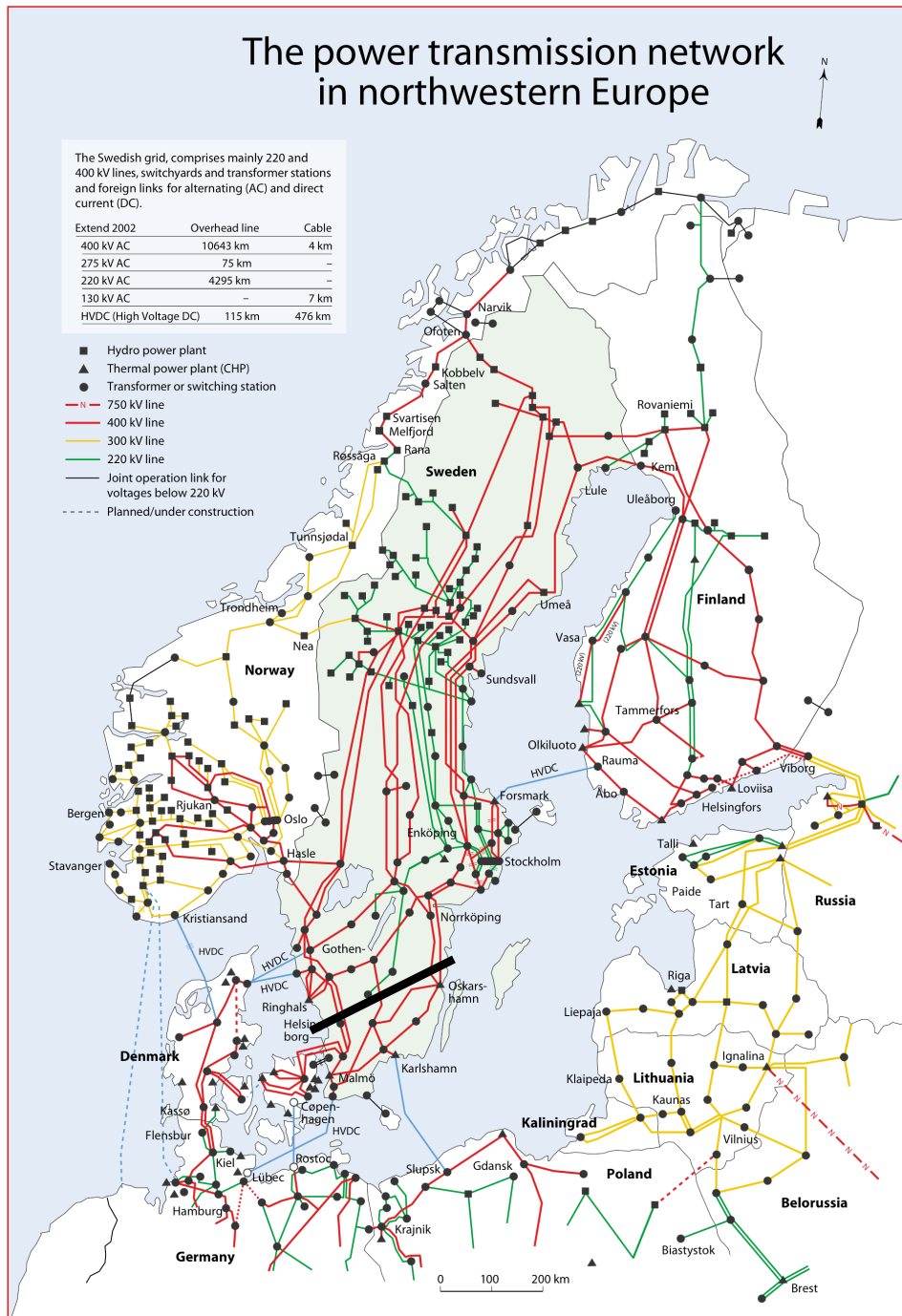
Fig. 1. The power transmission network in northwestern Europe. The line just north of Oskarshamn marks the modelled area.
